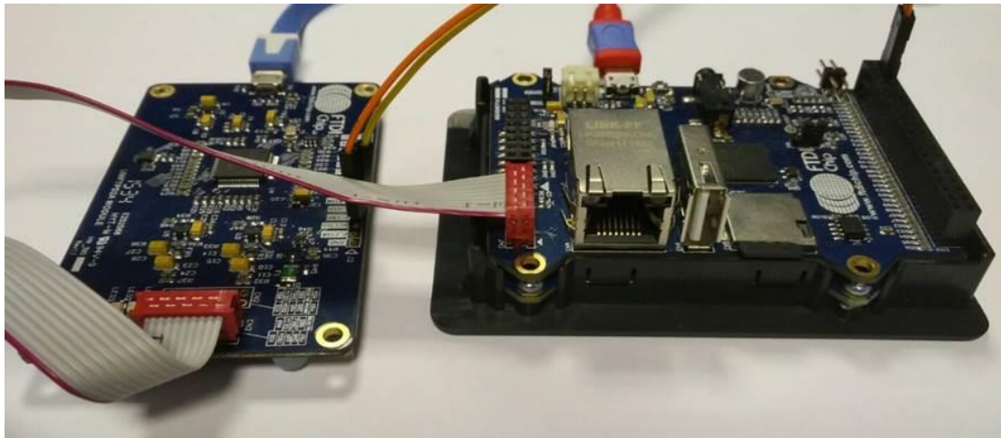
Figure 3.6 Hardware connections
