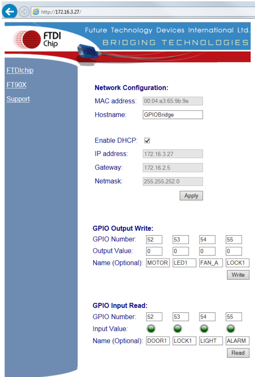
Figure 4.1 Web Configuration and Control Interface
