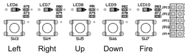
Figure 2.1.2: V-Eval Button Configuration
