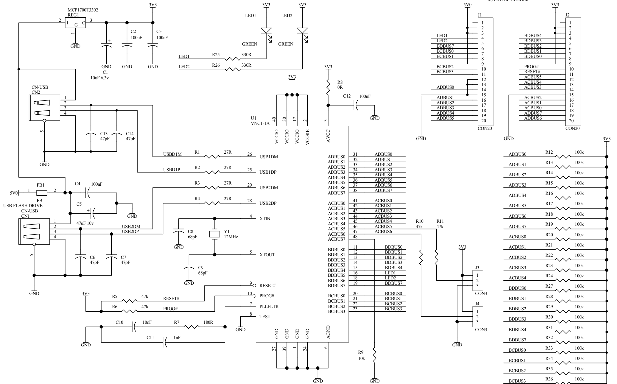
VINCULUM VDIP2 SCHEMATIC
