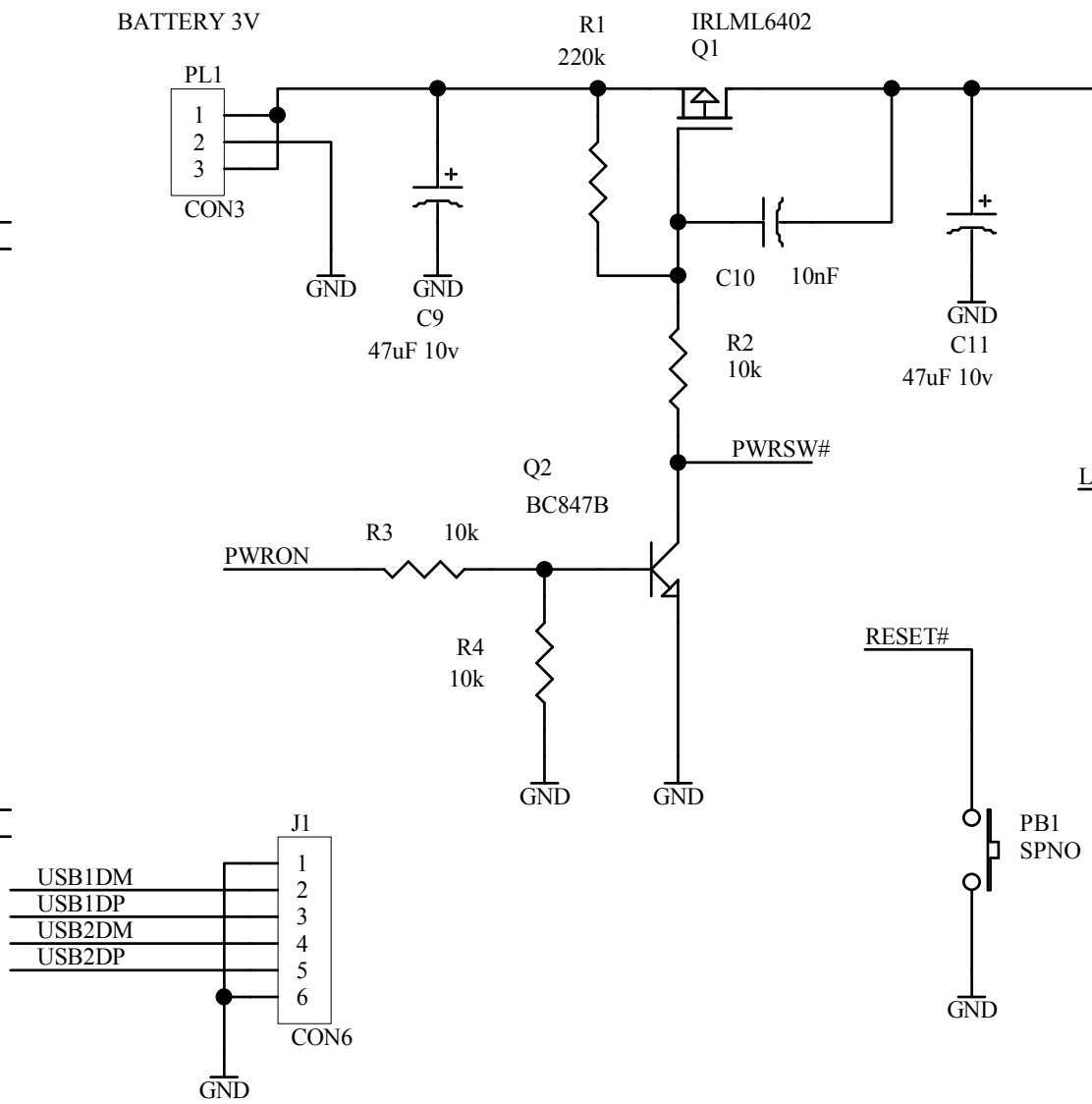
VINCULUM BACKUP FOR DIGITAL CAMERA / MP3 TO USB FLASH DRIVE SCHEMATIC ( A )
