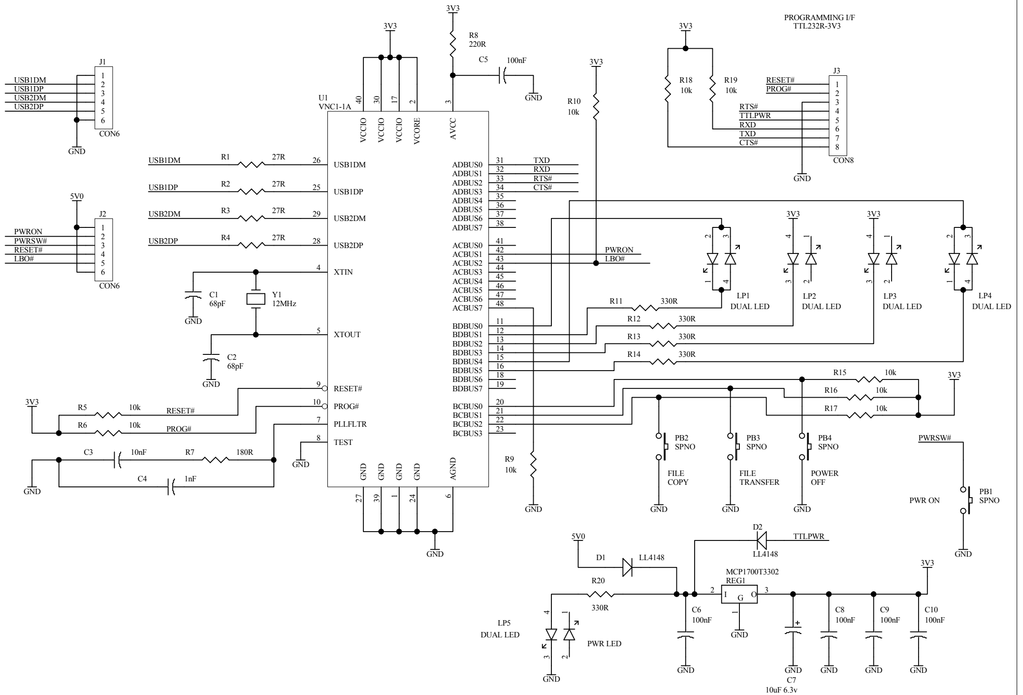
VINCULUM BACKUP FOR DIGITAL CAMERA / MP3 TO USB FLASH DRIVE SCHEMATIC ( B )
